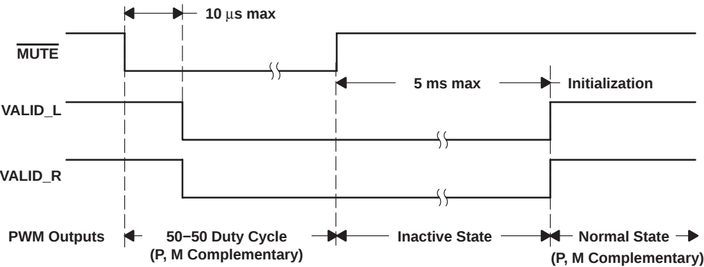
Figure 5. Mute Timing
