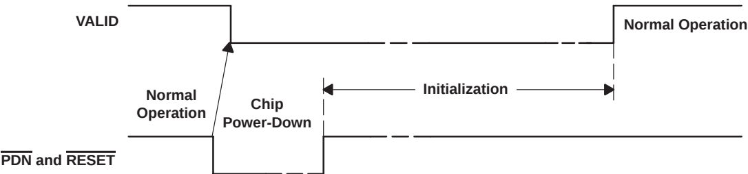
Figure 4. Power-Down Timing
